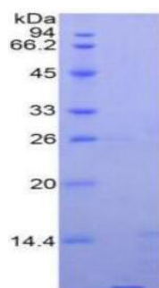
Figure. SDS-PAGE
