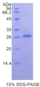
Figure. SDS-PAGE
