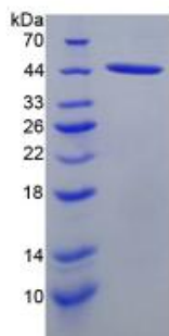
Figure. SDS-PAGE
